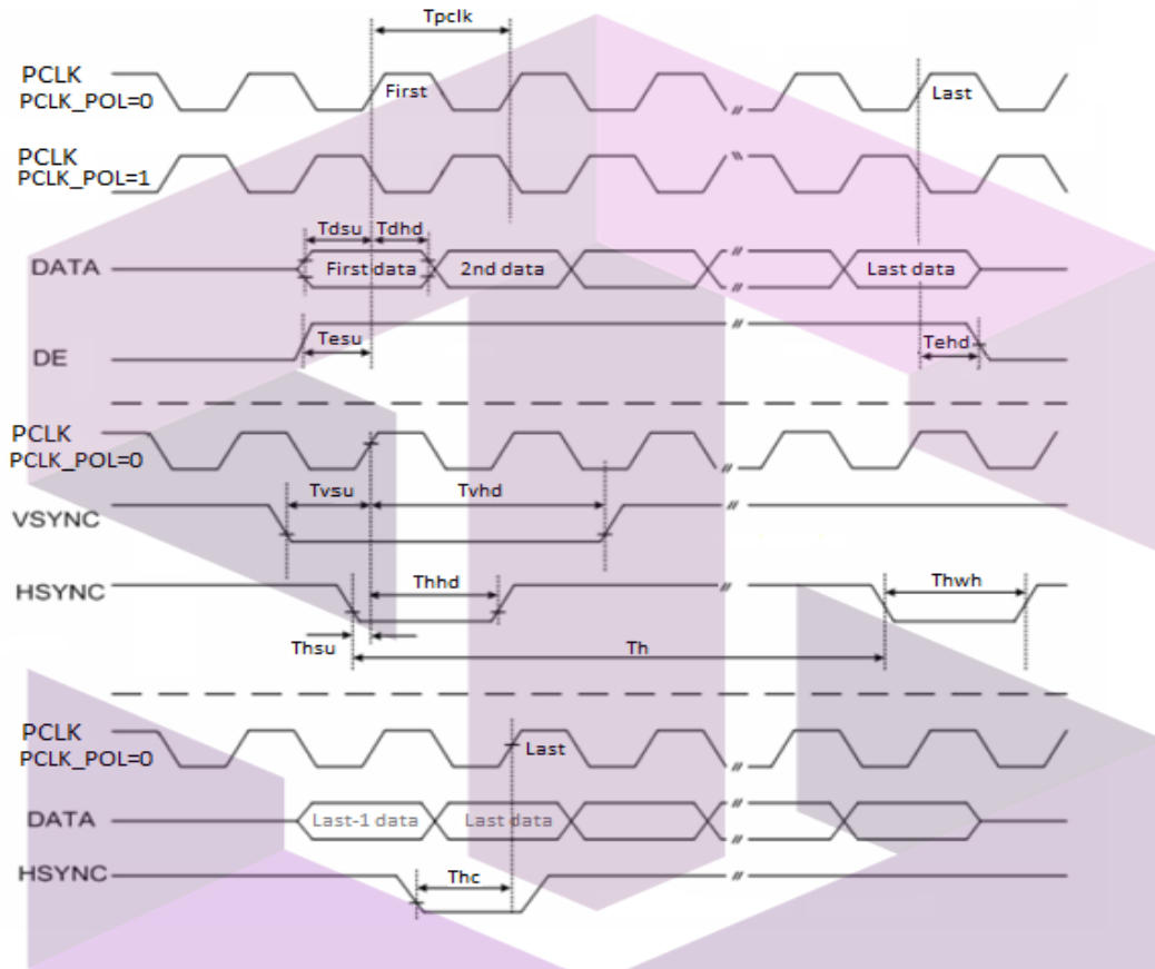
Figure 6-2 RGB Video Signal Timing
